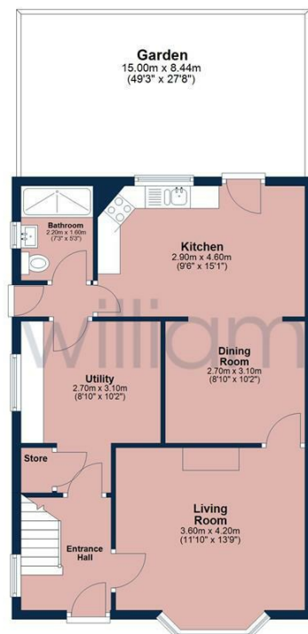
Ground Floor Approx. 54.2 sq. metres (583.1 sq. feet)
